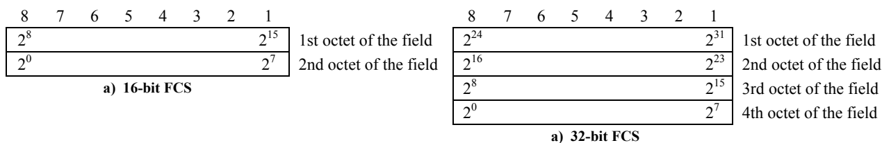
Figure 7/V.42 – FCS mapping convention
