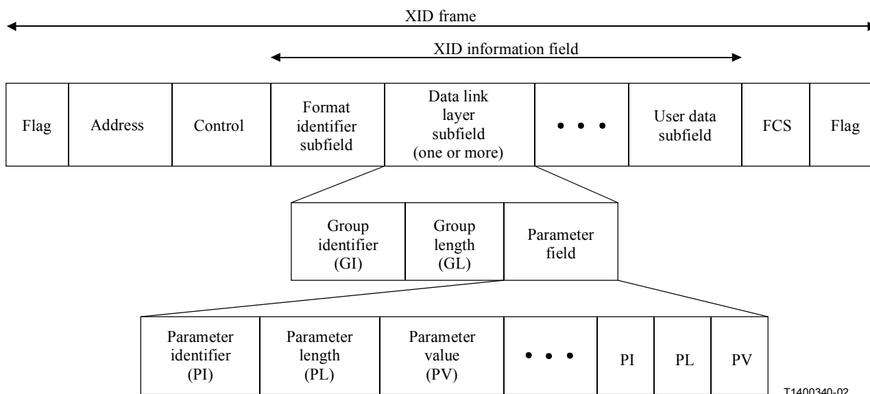
Figure 11/V.42 – General format of XID information field
